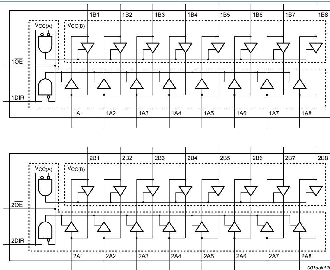
Fig. 2. Logic symbol
